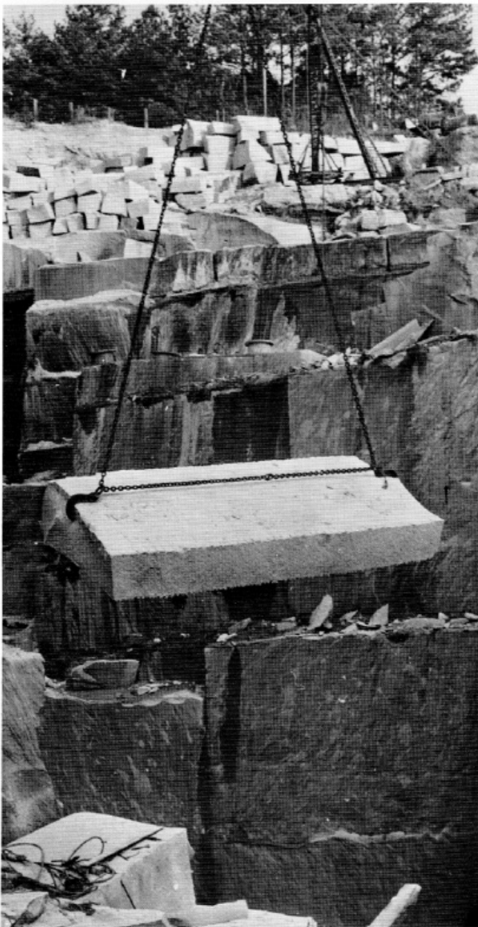
The first of The Georgia Guidestones ® blocks is lifted some 114 feet from the depths of Pyramid Quarry. Each block weighed approximately 28 tons.
