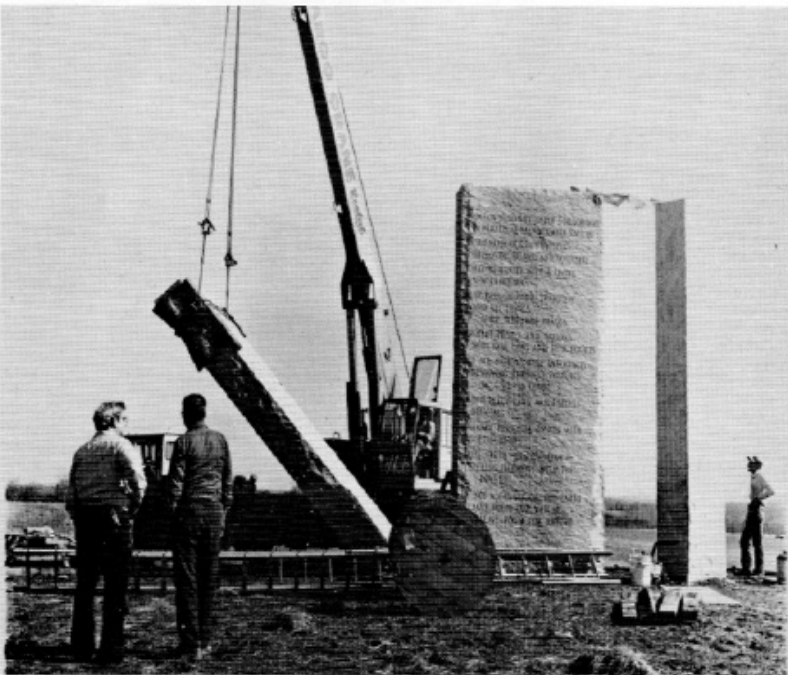
The third Guidestone is raised and about to be placed on the knoll alongside the first two stones. Looking over the erection procedure is Joe H. Fendley, Sr., builder of The Georgia Guidestones® and Joe B. Davis (l-r with back to camera), and Howard Davis (right), a member of the special crew who worked on the project.
