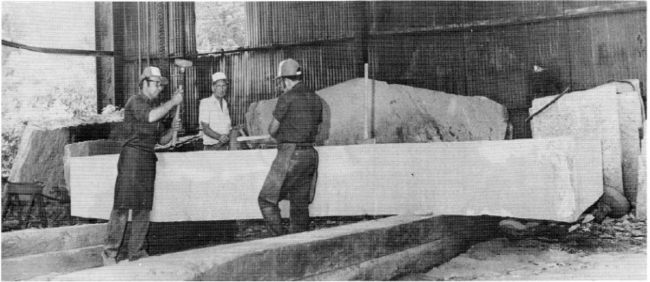
A special crew of Horace and Frankie Bradford, master stone craftsmen, under the direction of Joe B. Davis, background, a retired plant superintendent was hired to cut and pitch the granite slabs to the exact dimensions provided by "Mr. R.C. Christian." Special crews were hired because the project was so demanding that it would disrupt the regular Elberton Granite Finishing Company's production schedule.
