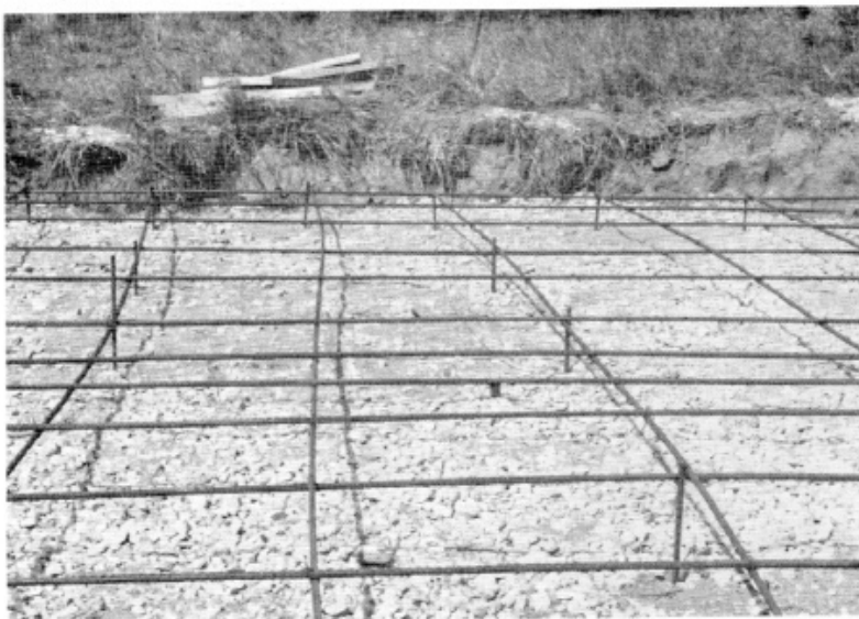
The foundation for The Georgia Guidestones was built on solid rock-bed, and the cement was mixed according to rigid specifications and reinforced with steel, as shown in the photograph above. All according to the Sponsor's instructions.
